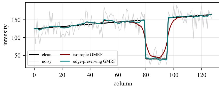
(h) Row 40 profile: edge sharpness
