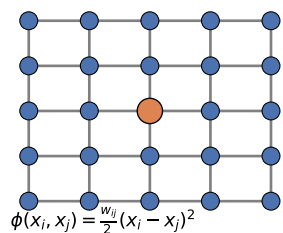
(e) 4-connected MRF graph
